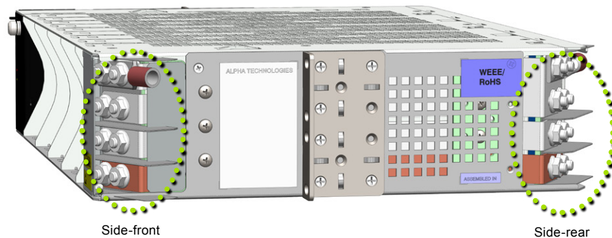
Figure 3 LPS36 Input 48Vdc Connections
