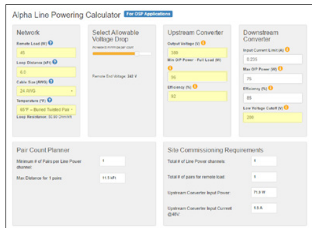
Figure 3 Line Power Calculator Results for Example #1
