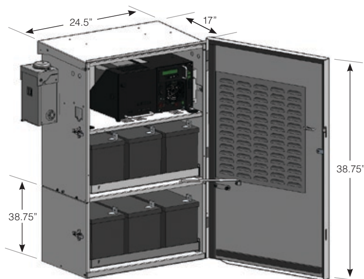
UBE-PWE Dimensions
